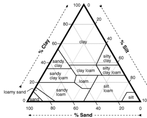
The Soil Texture Pyramid
