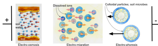
Electrokinetic Processes in a DC Field
