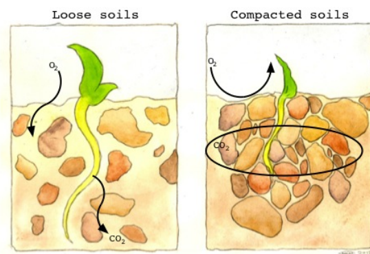
Differences Between Loose and Compacted Soils
